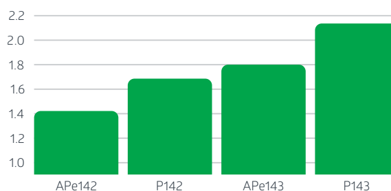
Air consumption m 3 /h at 2 bar
